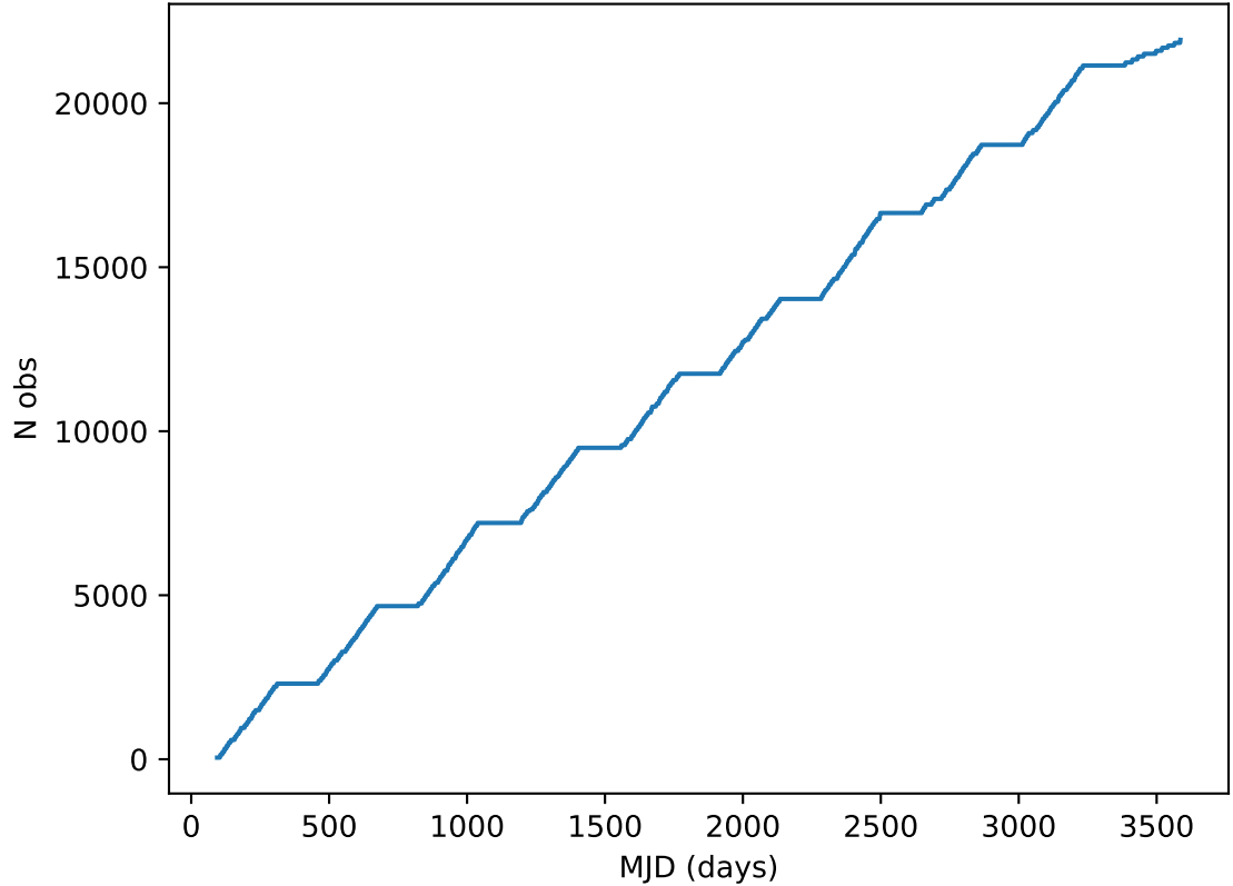
too_elab_heavy_r128_d2_ugrizy_v3.4_10yrs all bands: DD:ECDFS Cumulative NVisits
