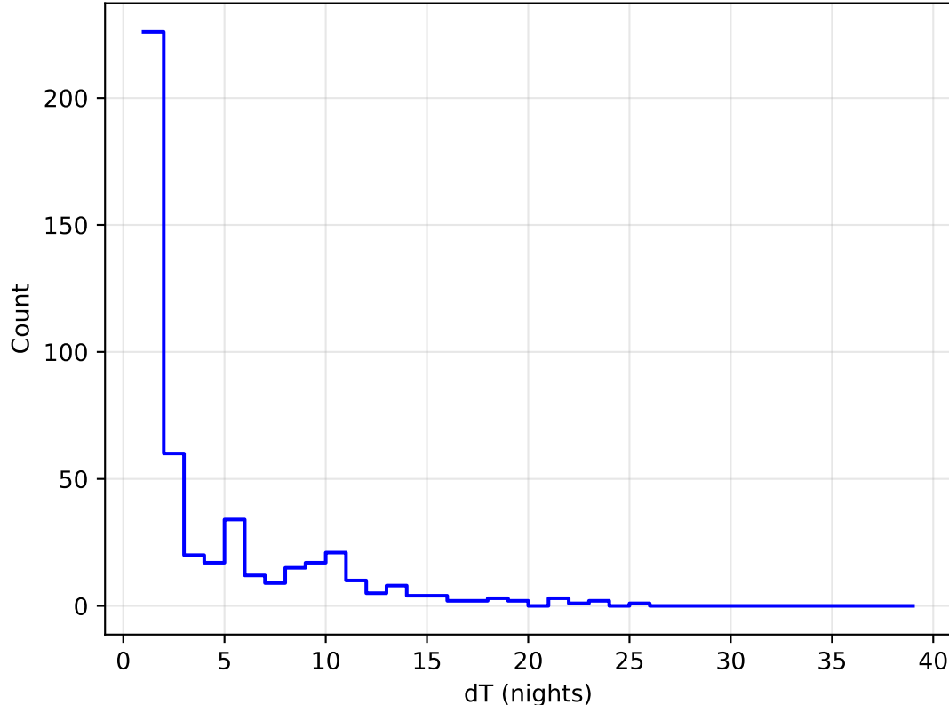
too_elab_heavy_r128_d2_ugrizy_v3.4_10yrs all bands: DD: COSMOS Delta Nights Histogram
