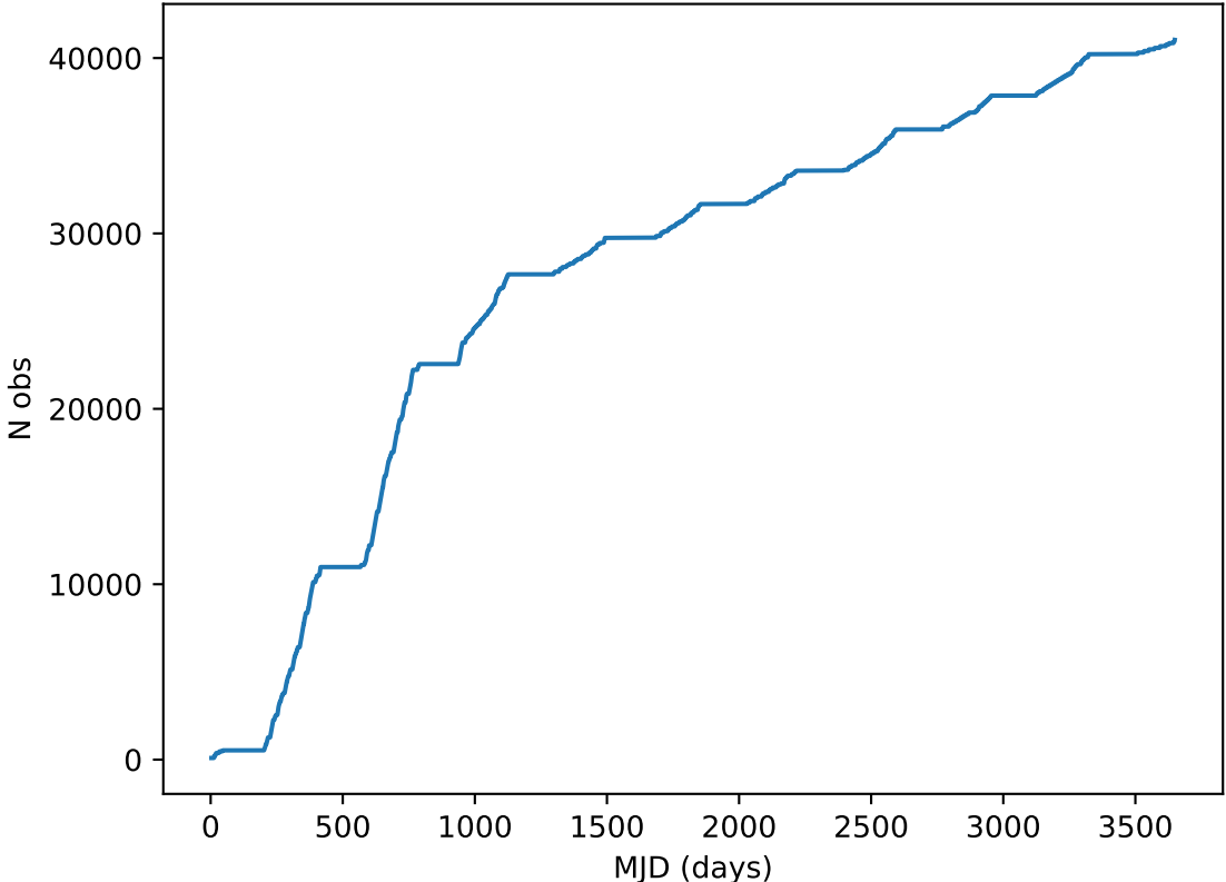
too_elab_heavy_r128_d2_ugrizy_v3.4_10yrs all bands: DD: COSMOS Cumulative NVisits
