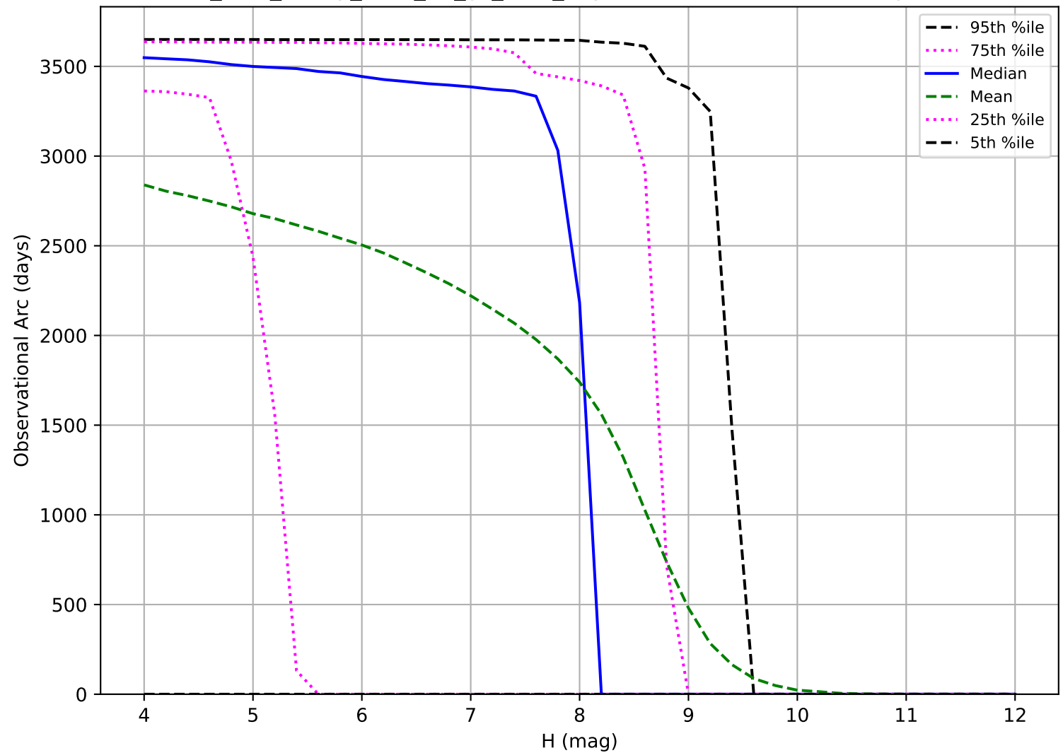
too_elab_heavy_r128_d2_gz_v3.4_10yrs: Observational Arc Length TNO
