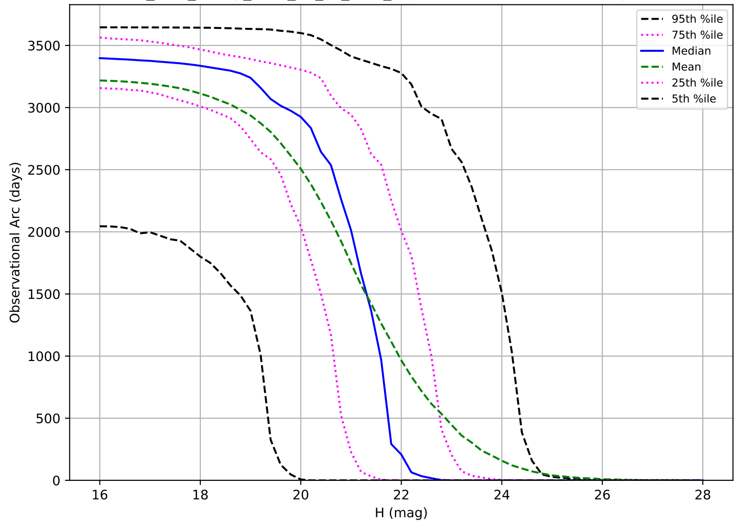
too_elab_heavy_r128_d2_gz_v3.4_10yrs: Observational Arc Length PHA
