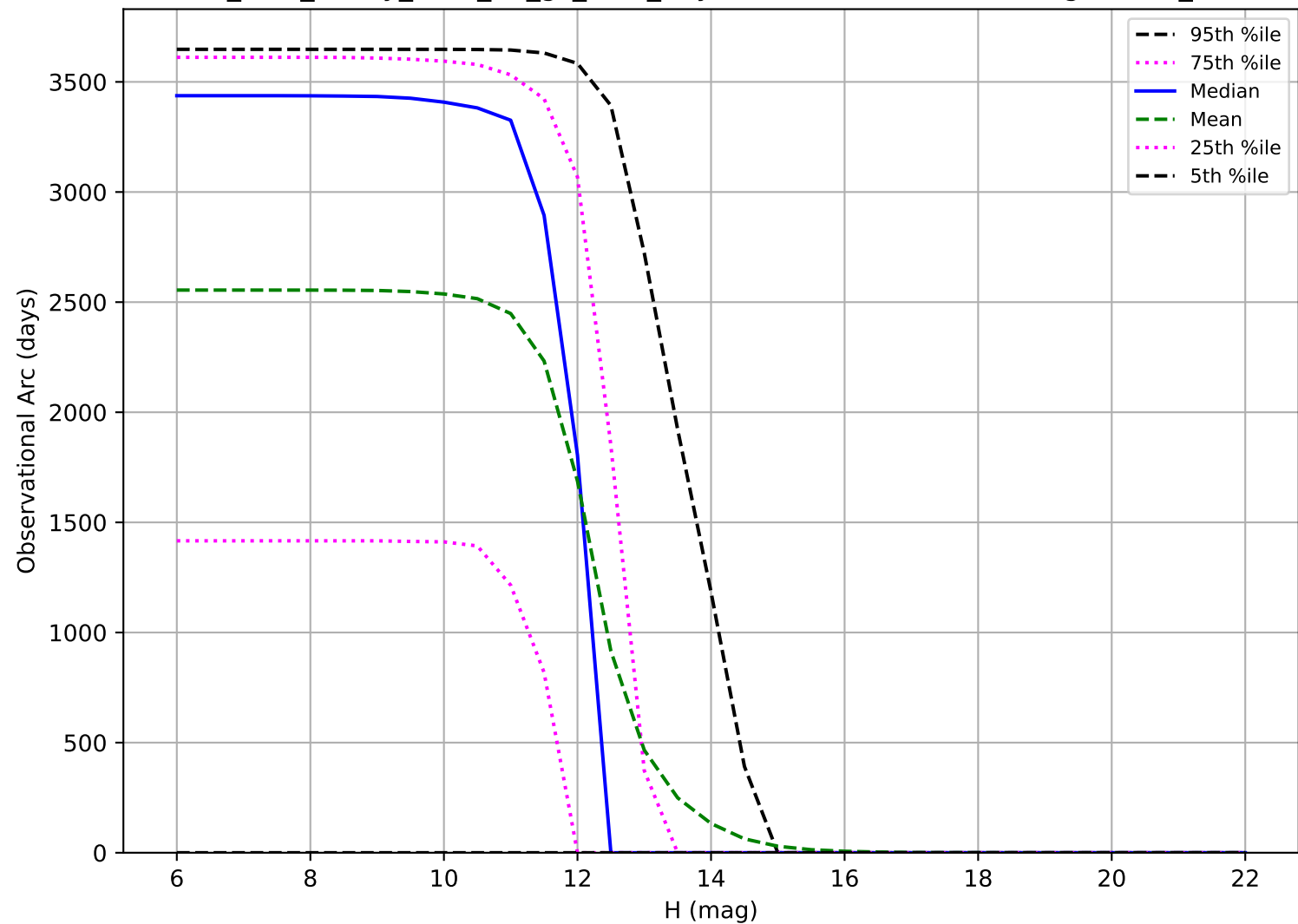
too_elab_heavy_r128_d2_gz_v3.4_10yrs: Observational Arc Length OCC_r20
