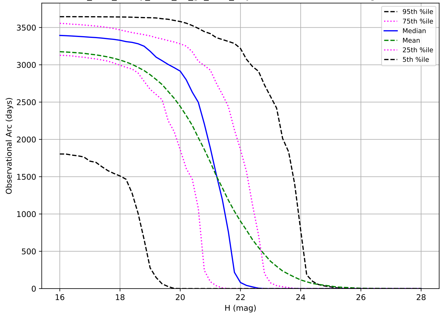
too_elab_heavy_r128_d2_gz_v3.4_10yrs: Observational Arc Length NEO
