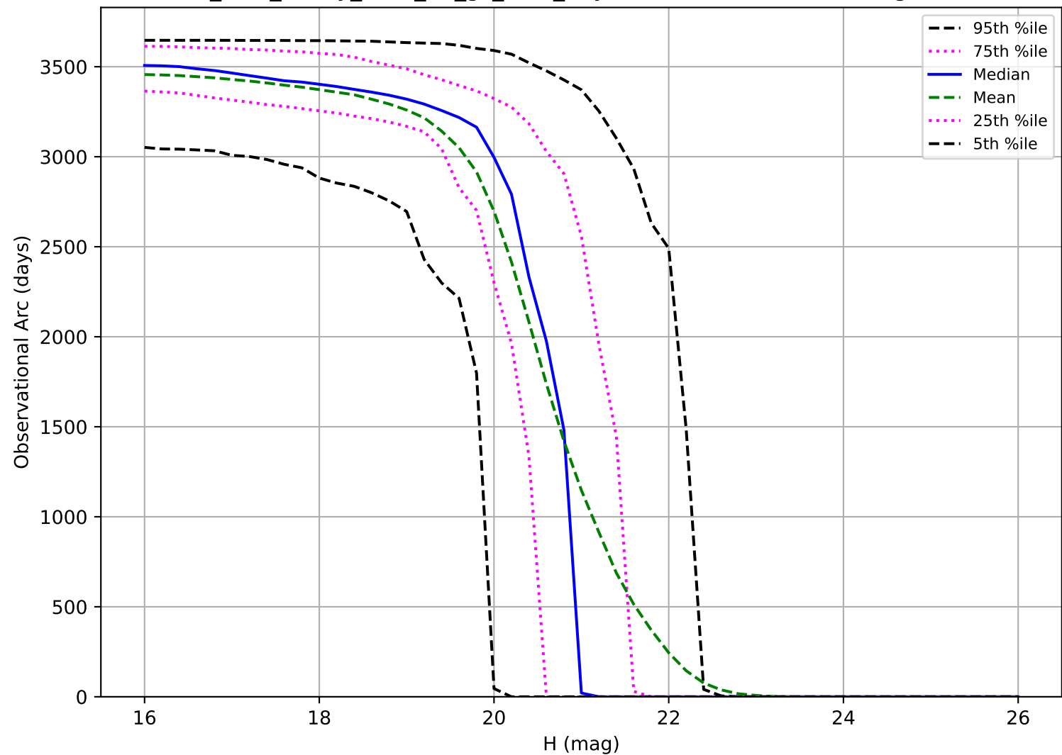
too_elab_heavy_r128_d2_gz_v3.4_10yrs: Observational Arc Length MBA
