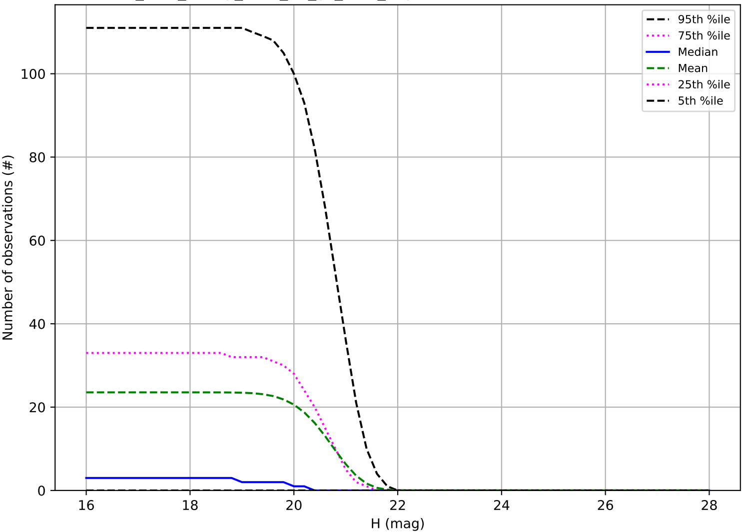
too_elab_heavy_r128_d2_gz_v3.4_10yrs: Number of observations Vatira
