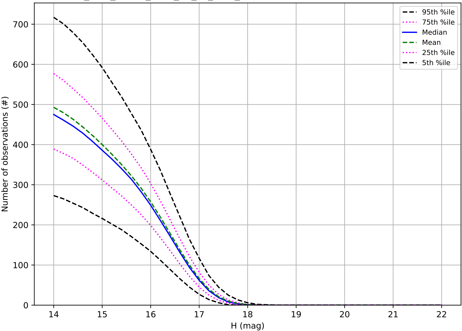
too_elab_heavy_r128_d2_gz_v3.4_10yrs: Number of observations Trojan
