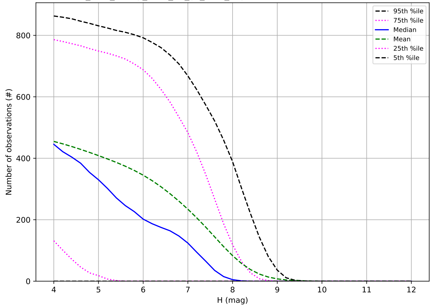
too_elab_heavy_r128_d2_gz_v3.4_10yrs: Number of observations TNO
