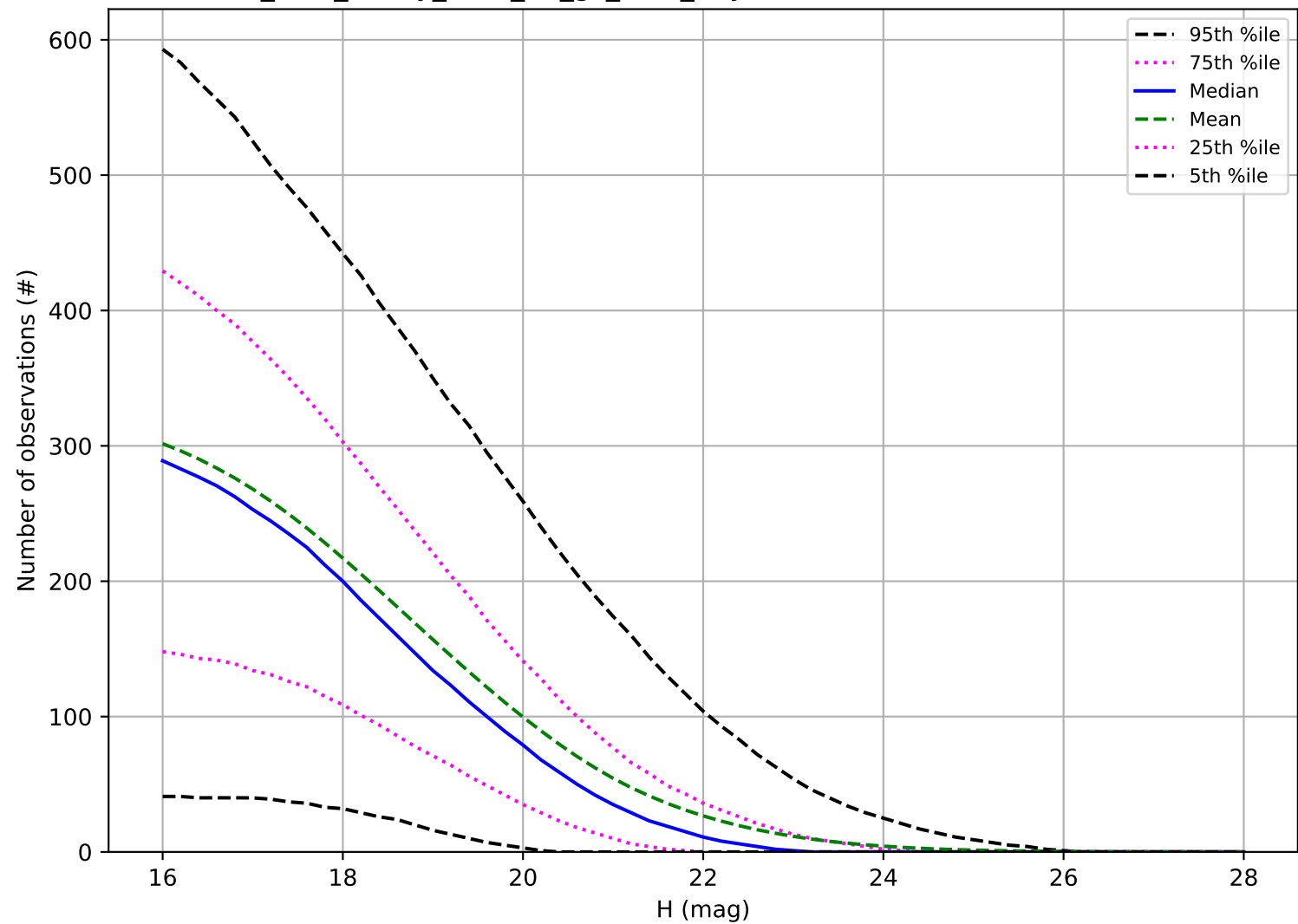
too_elab_heavy_r128_d2_gz_v3.4_10yrs: Number of observations PHA
