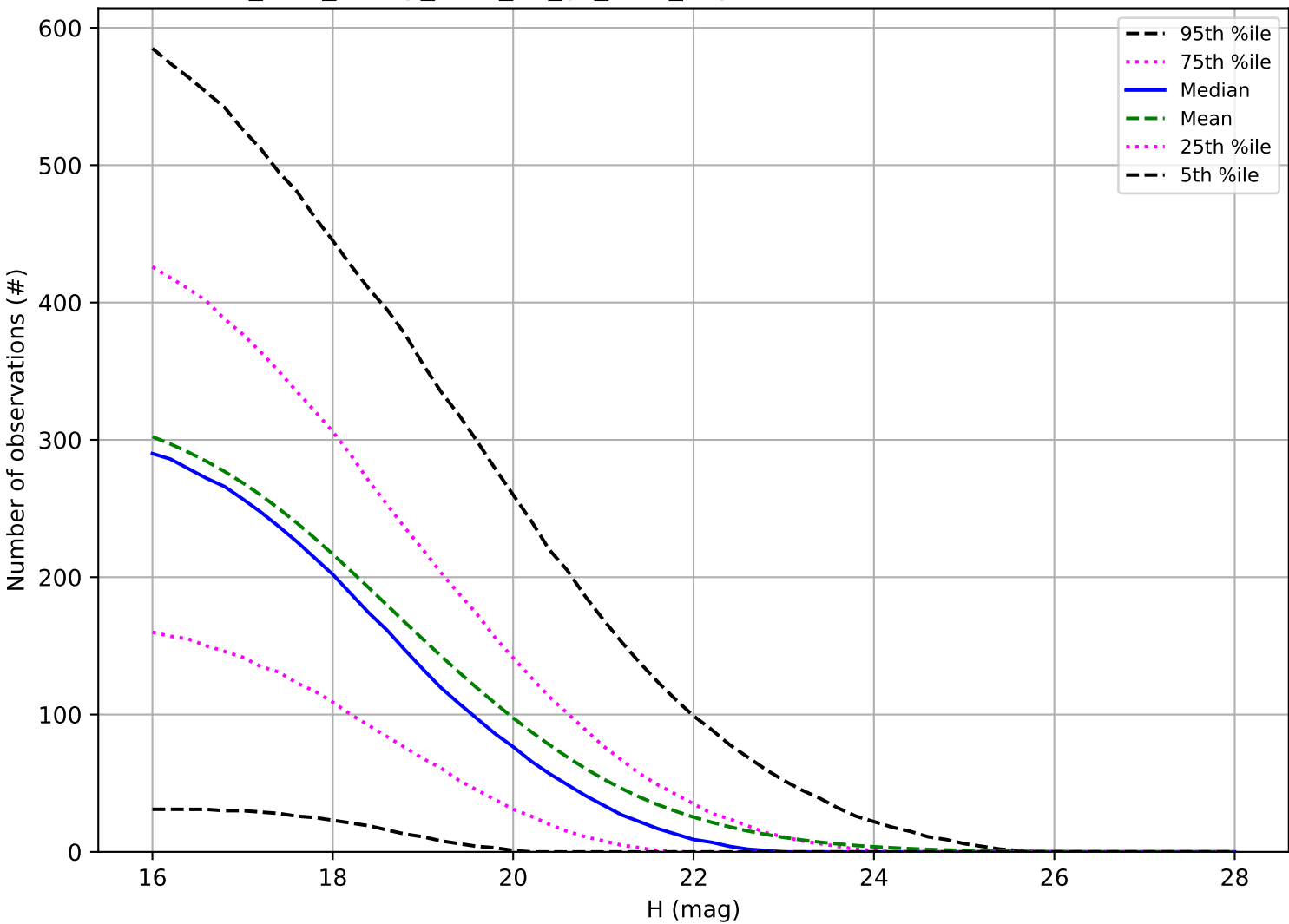
too_elab_heavy_r128_d2_gz_v3.4_10yrs: Number of observations NEO
