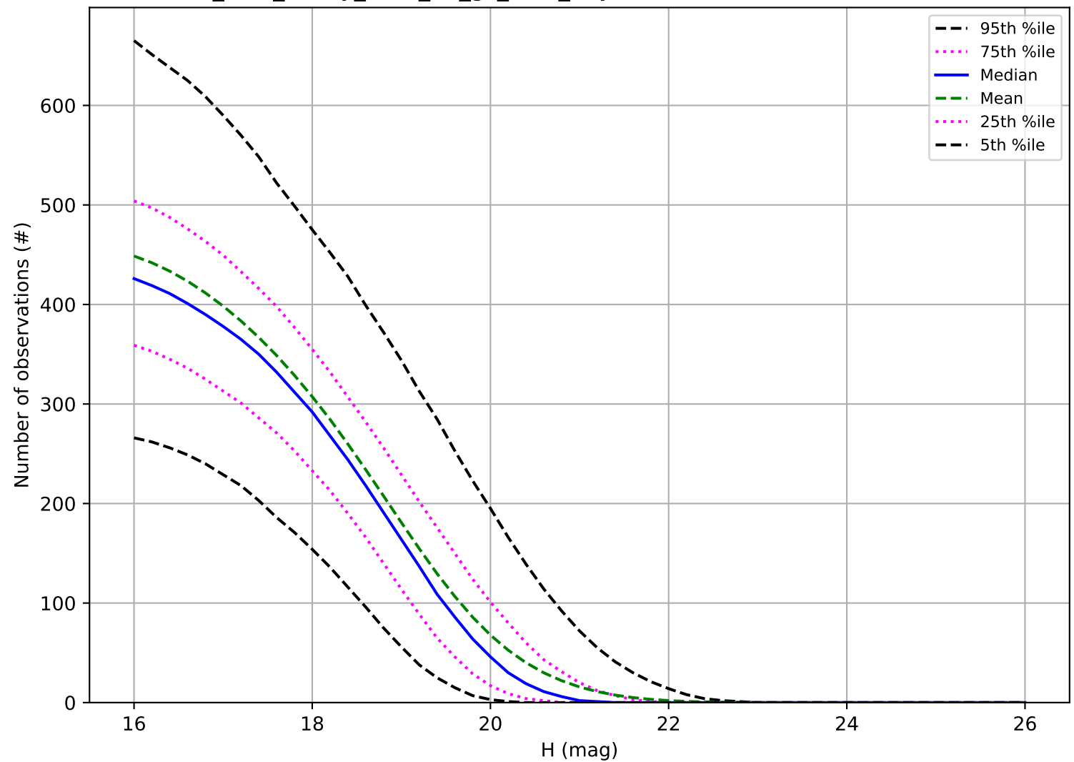
too_elab_heavy_r128_d2_gz_v3.4_10yrs: Number of observations MBA
