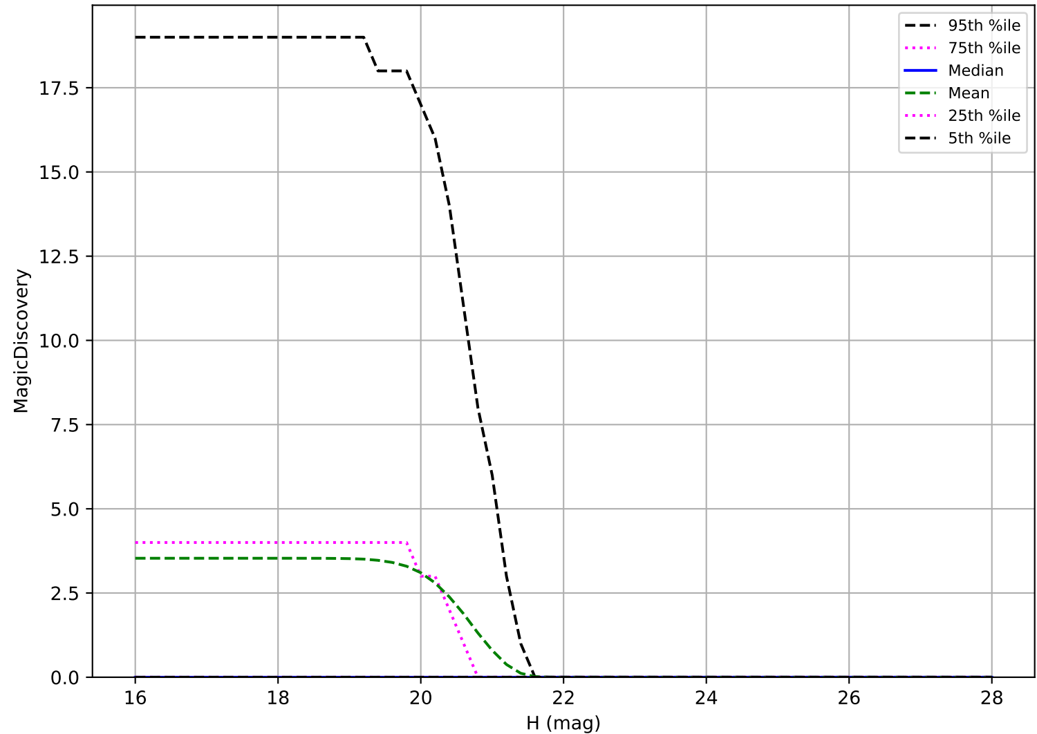
too_elab_heavy_r128_d2_gz_v3.4_10yrs: Vatira 6 detections in 60 nights detection loss
