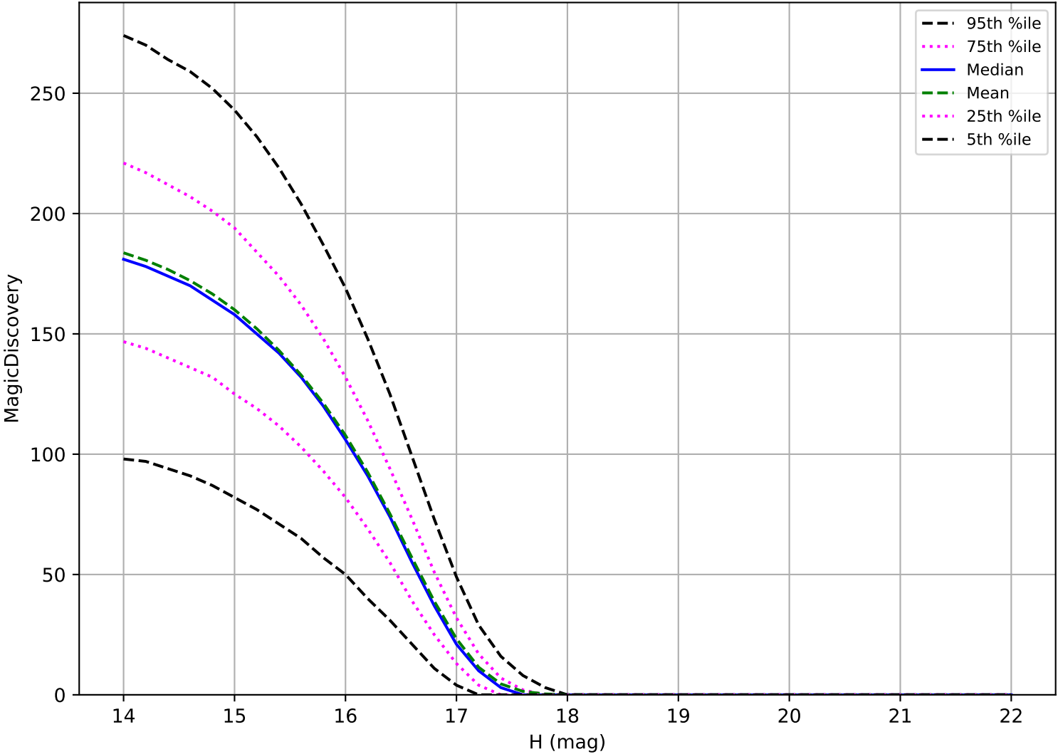
too_elab_heavy_r128_d2_gz_v3.4_10yrs: Trojan 6 detections in 60 nights detection loss
