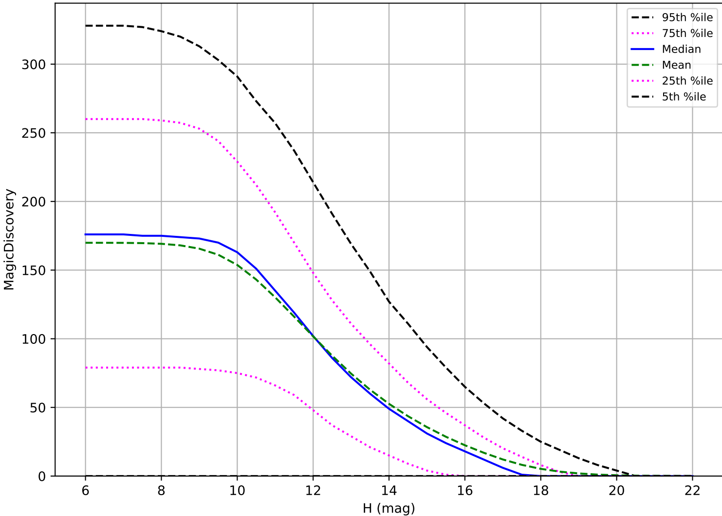
too_elab_heavy_r128_d2_gz_v3.4_10yrs: OCC_r5 6 detections in 60 nights detection loss
