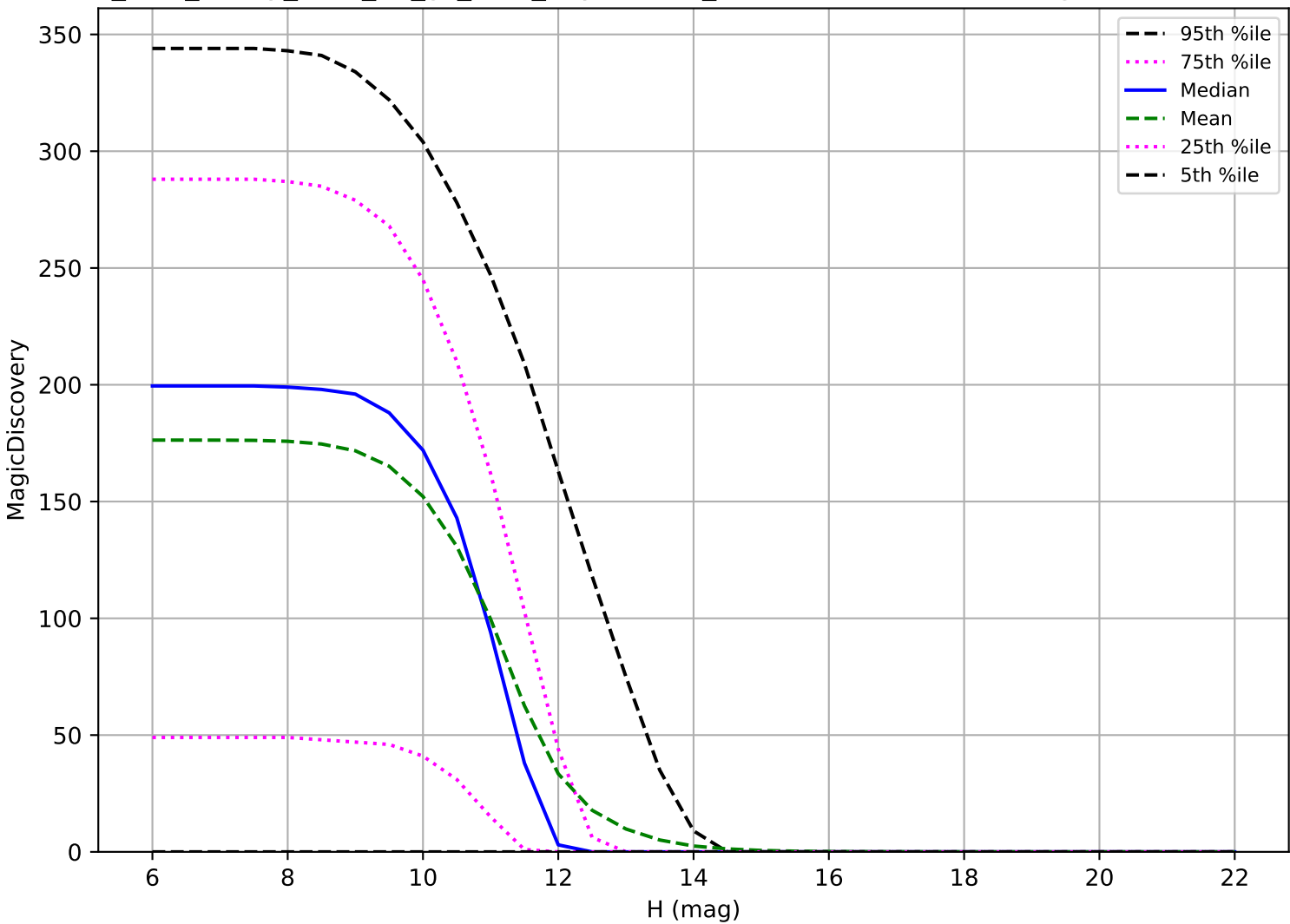
too_elab_heavy_r128_d2_gz_v3.4_10yrs: OCC_r20 6 detections in 60 nights detection loss
