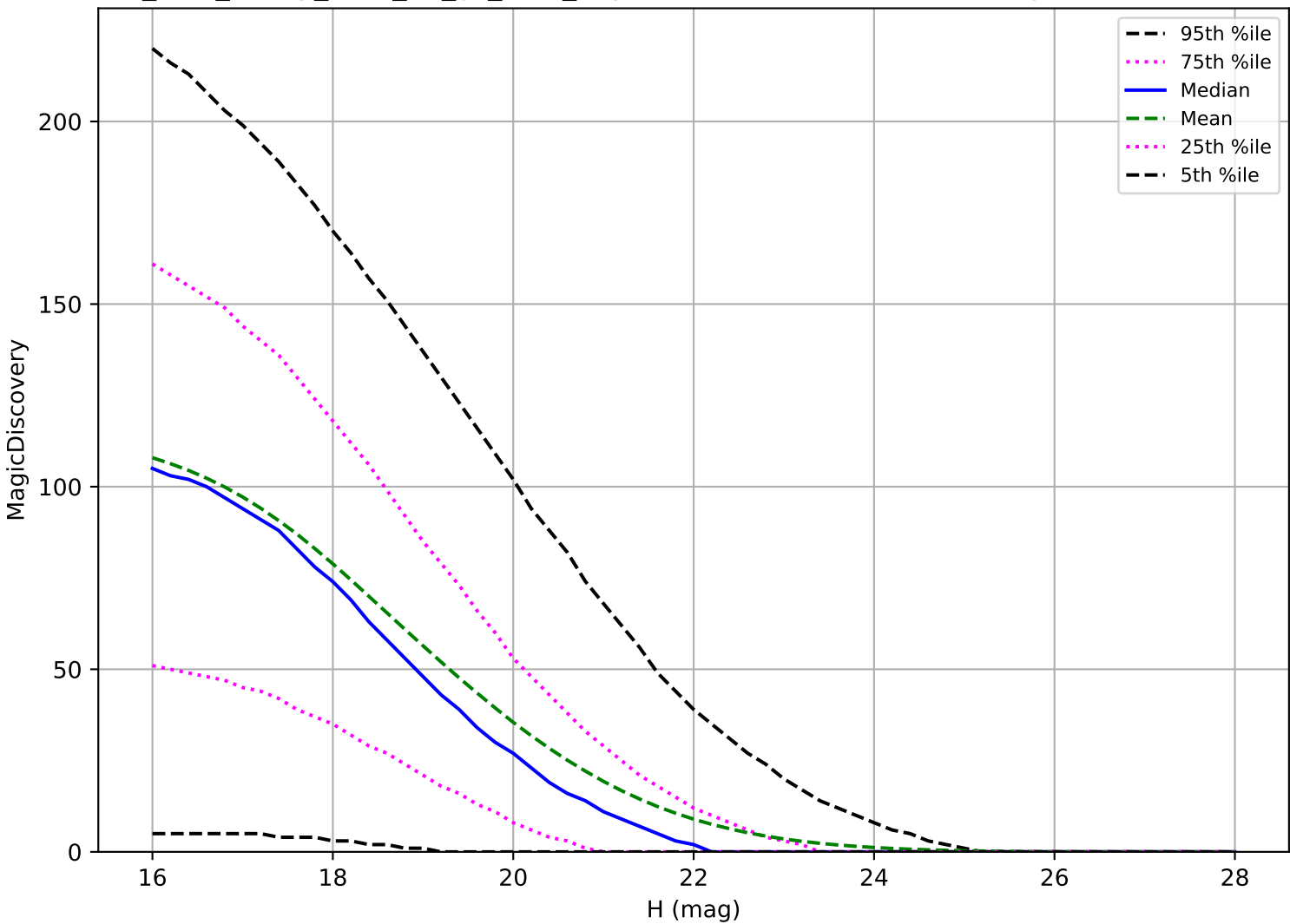
too_elab_heavy_r128_d2_gz_v3.4_10yrs: NEO 6 detections in 60 nights detection loss
