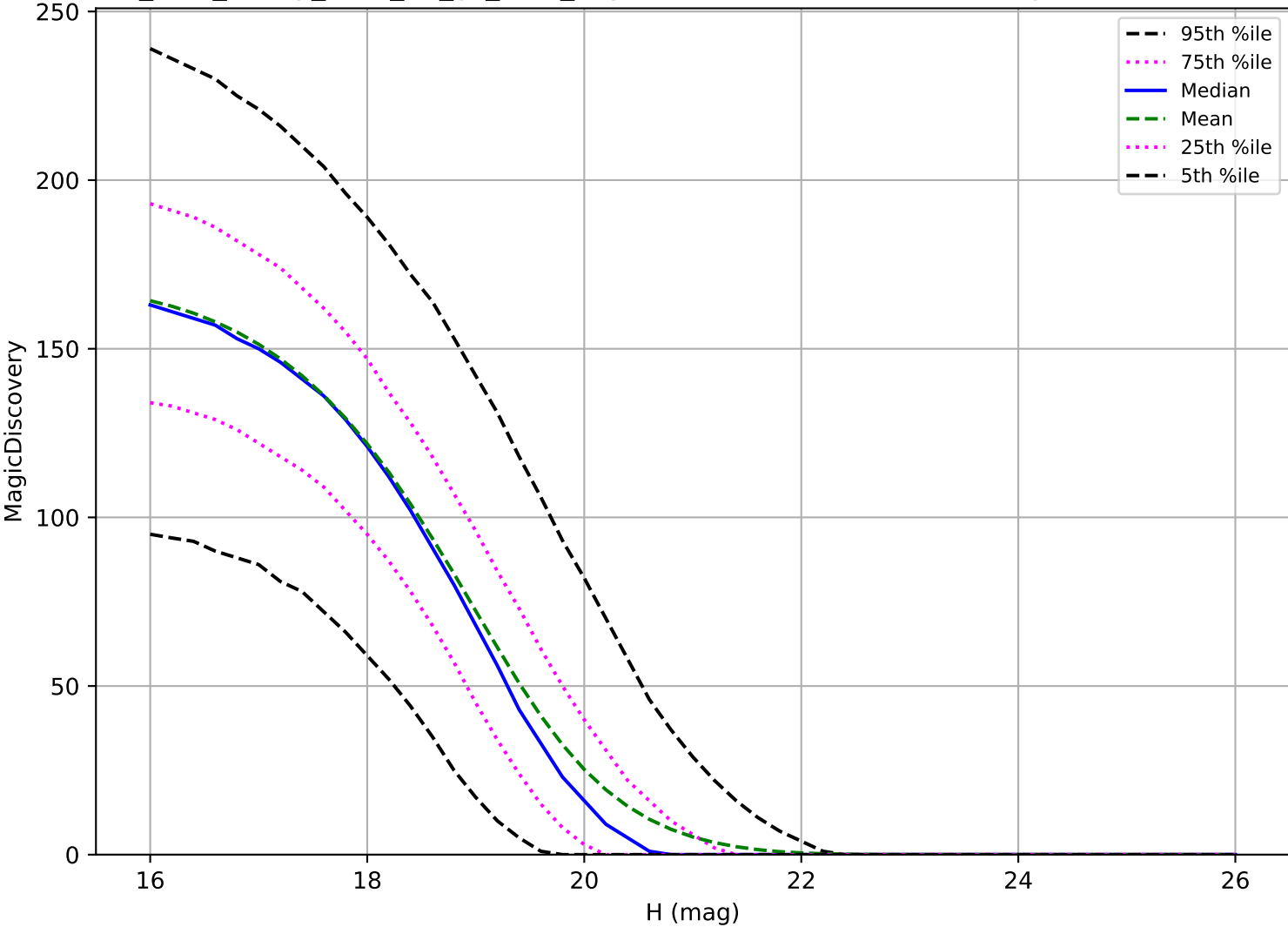
too_elab_heavy_r128_d2_gz_v3.4_10yrs: MBA 6 detections in 60 nights detection loss
