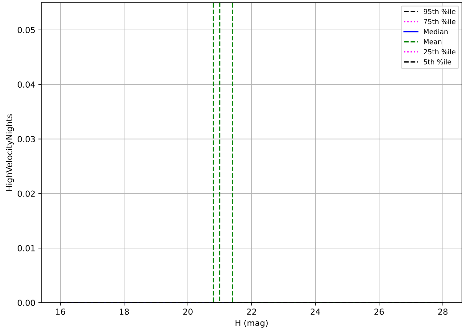
too_elab_heavy_r128_d2_gz_v3.4_10yrs: Vatira High velocity pair detection loss
