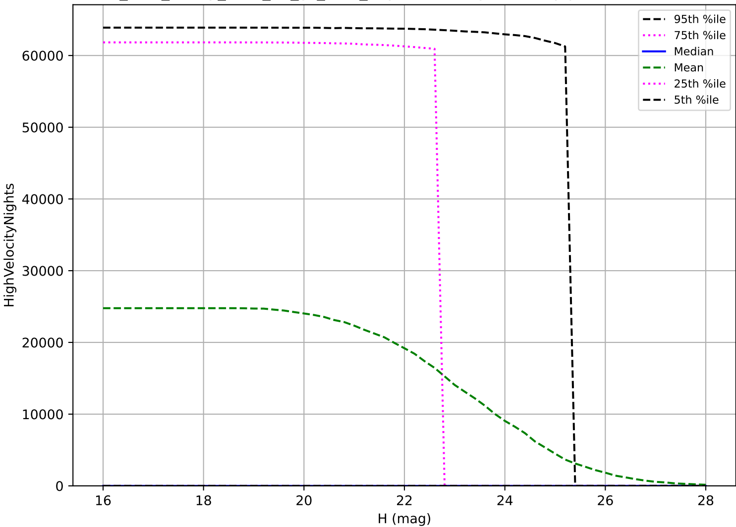
too_elab_heavy_r128_d2_gz_v3.4_10yrs: PHA High velocity pair detection loss
