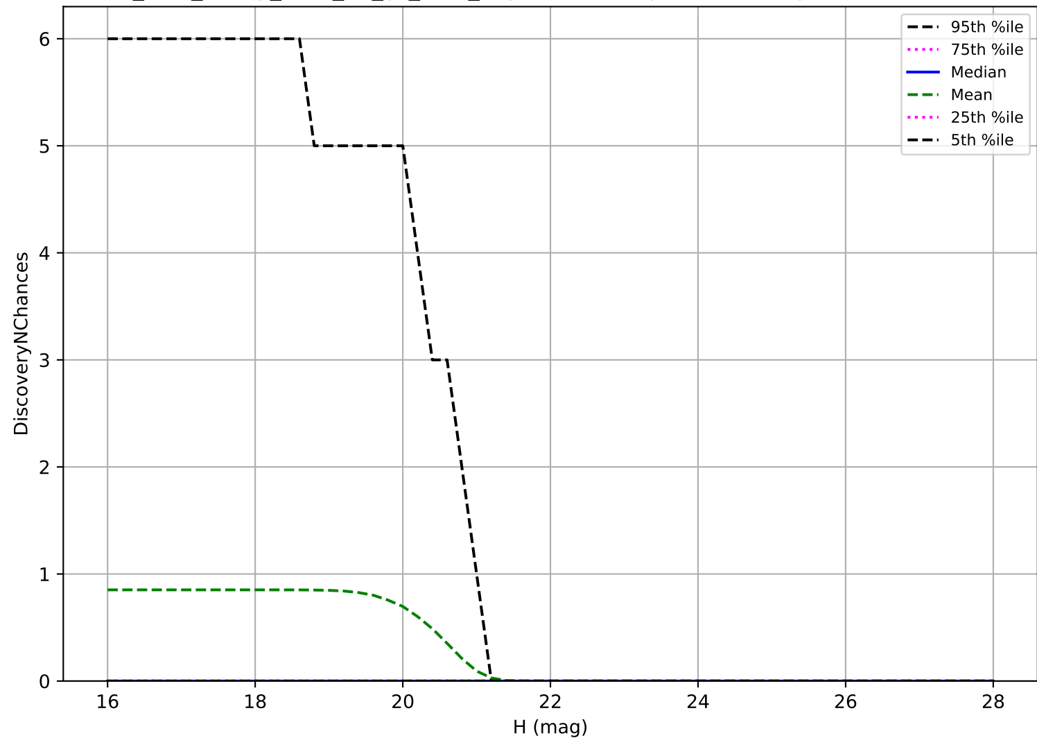
too_elab_heavy_r128_d2_gz_v3.4_10yrs: Vatira 3 pairs in 15 nights detection loss
