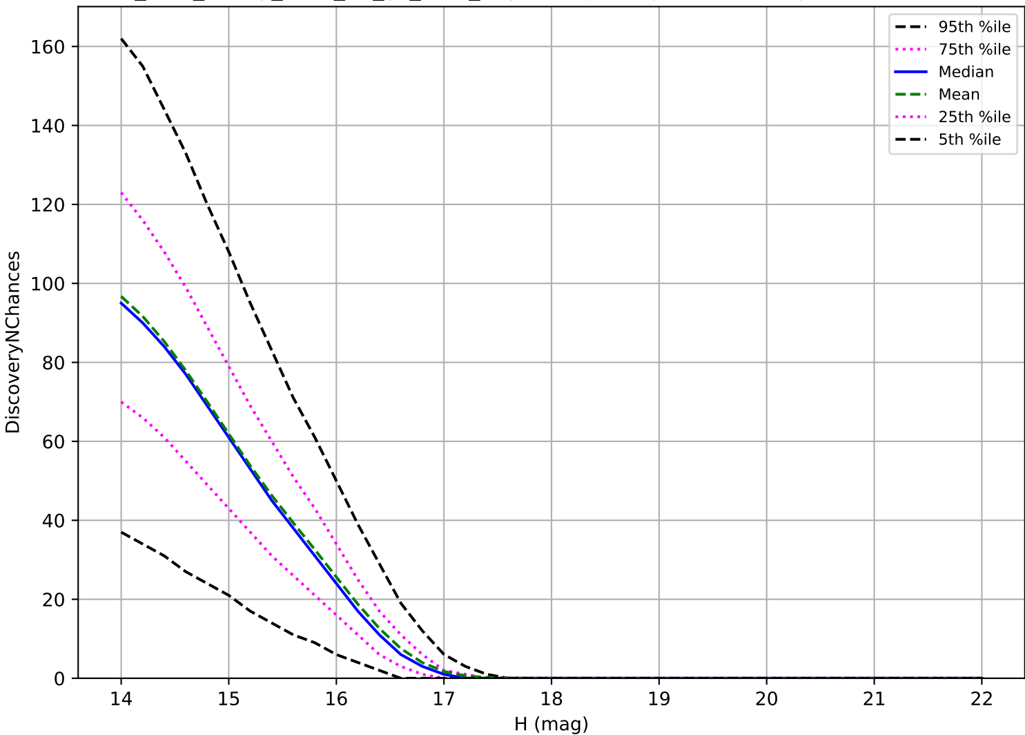
too_elab_heavy_r128_d2_gz_v3.4_10yrs: Trojan 3 pairs in 15 nights detection loss
