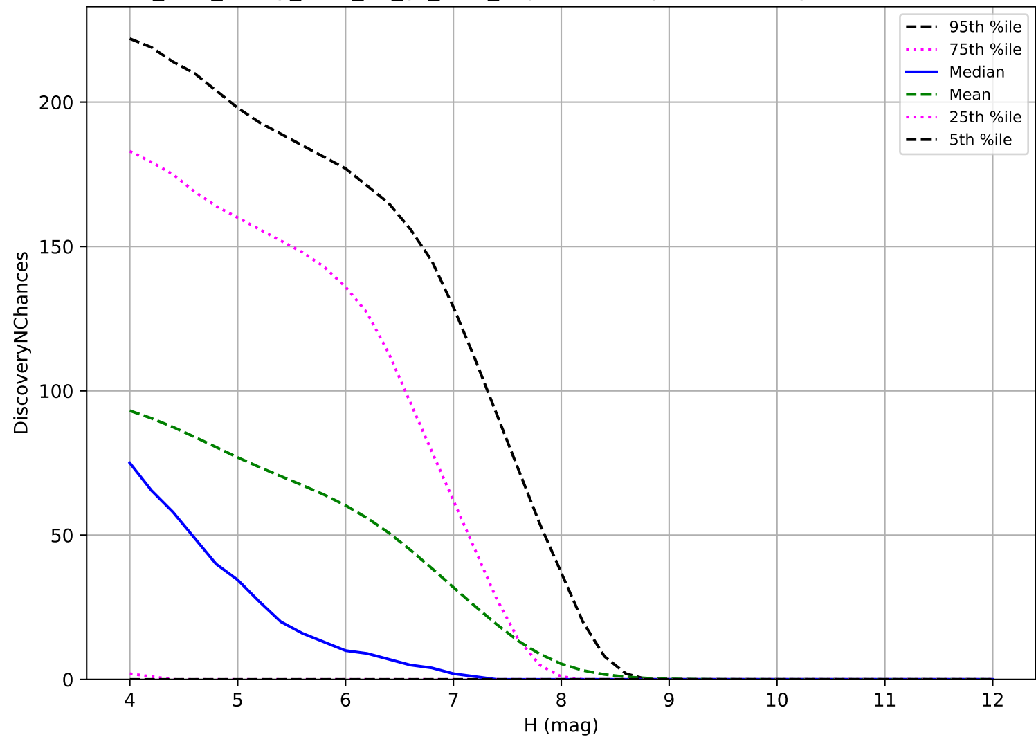
too_elab_heavy_r128_d2_gz_v3.4_10yrs: TNO 3 pairs in 15 nights detection loss
