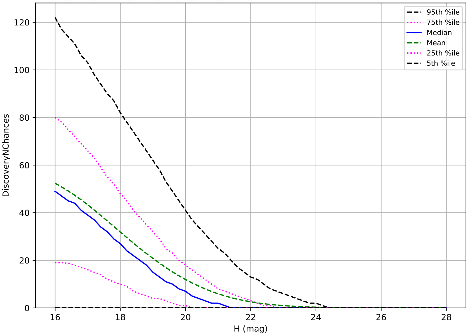
too_elab_heavy_r128_d2_gz_v3.4_10yrs: NEO 3 pairs in 15 nights detection loss
