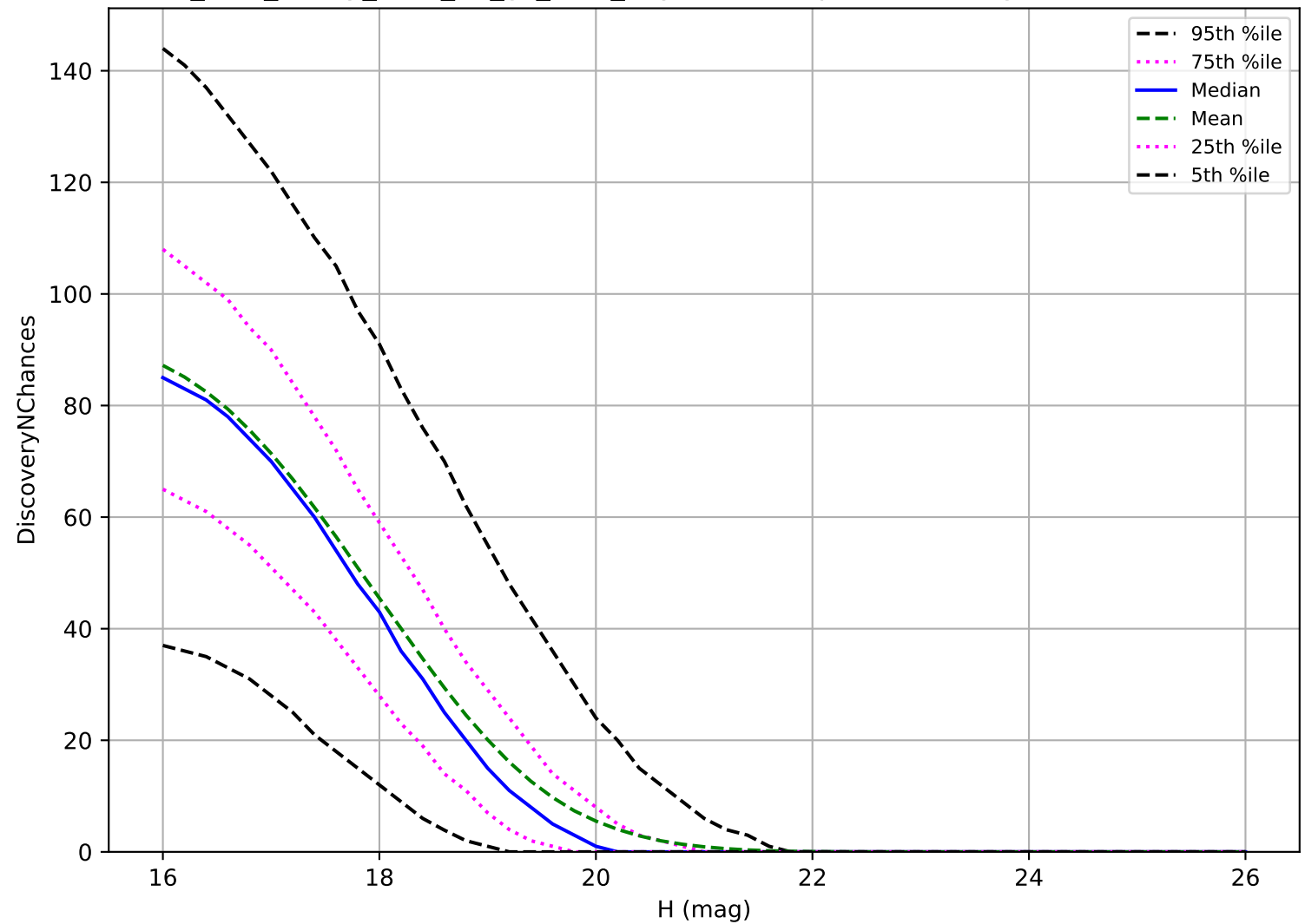
too_elab_heavy_r128_d2_gz_v3.4_10yrs: MBA 3 pairs in 15 nights detection loss
