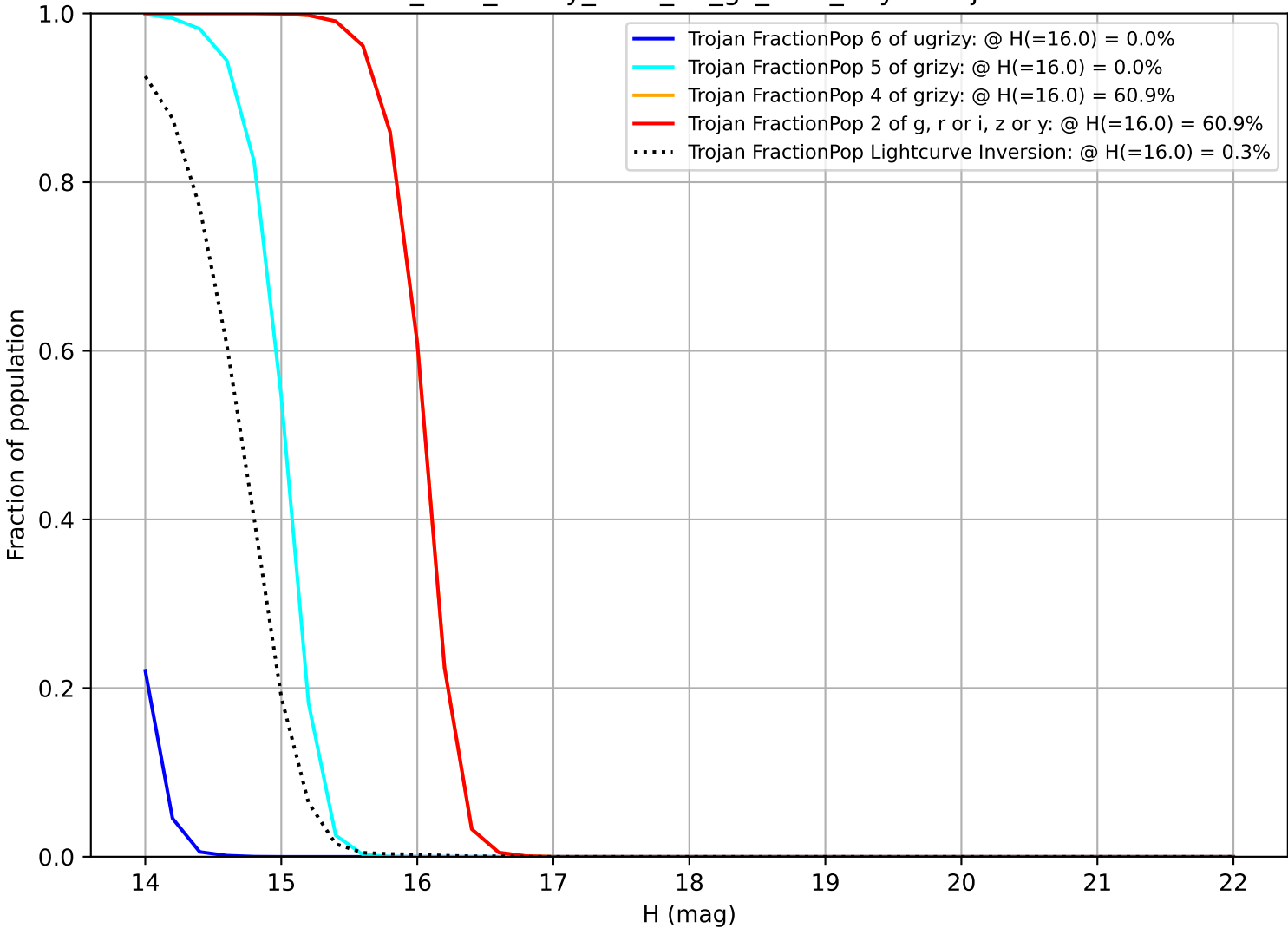
too_elab_heavy_r128_d2_gz_v3.4_10yrs Trojan
