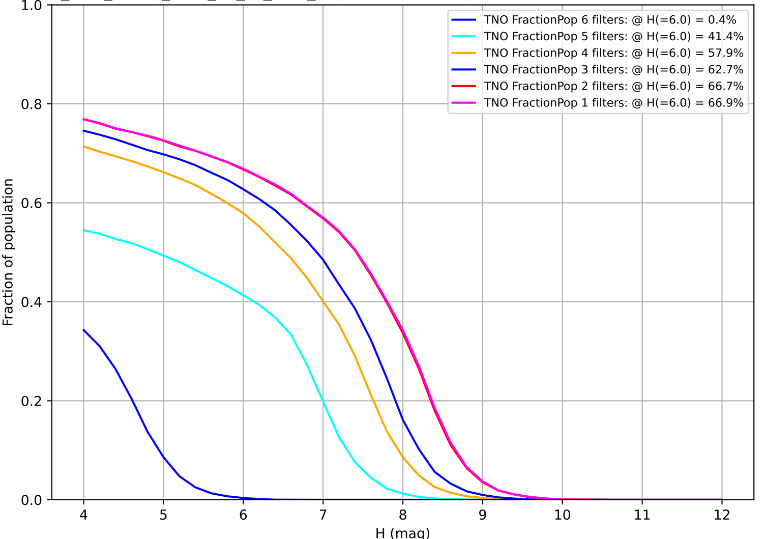
too_elab_heavy_r128_d2_gz_v3.4_10yrs: Fraction of population with colors in X filters TNO
