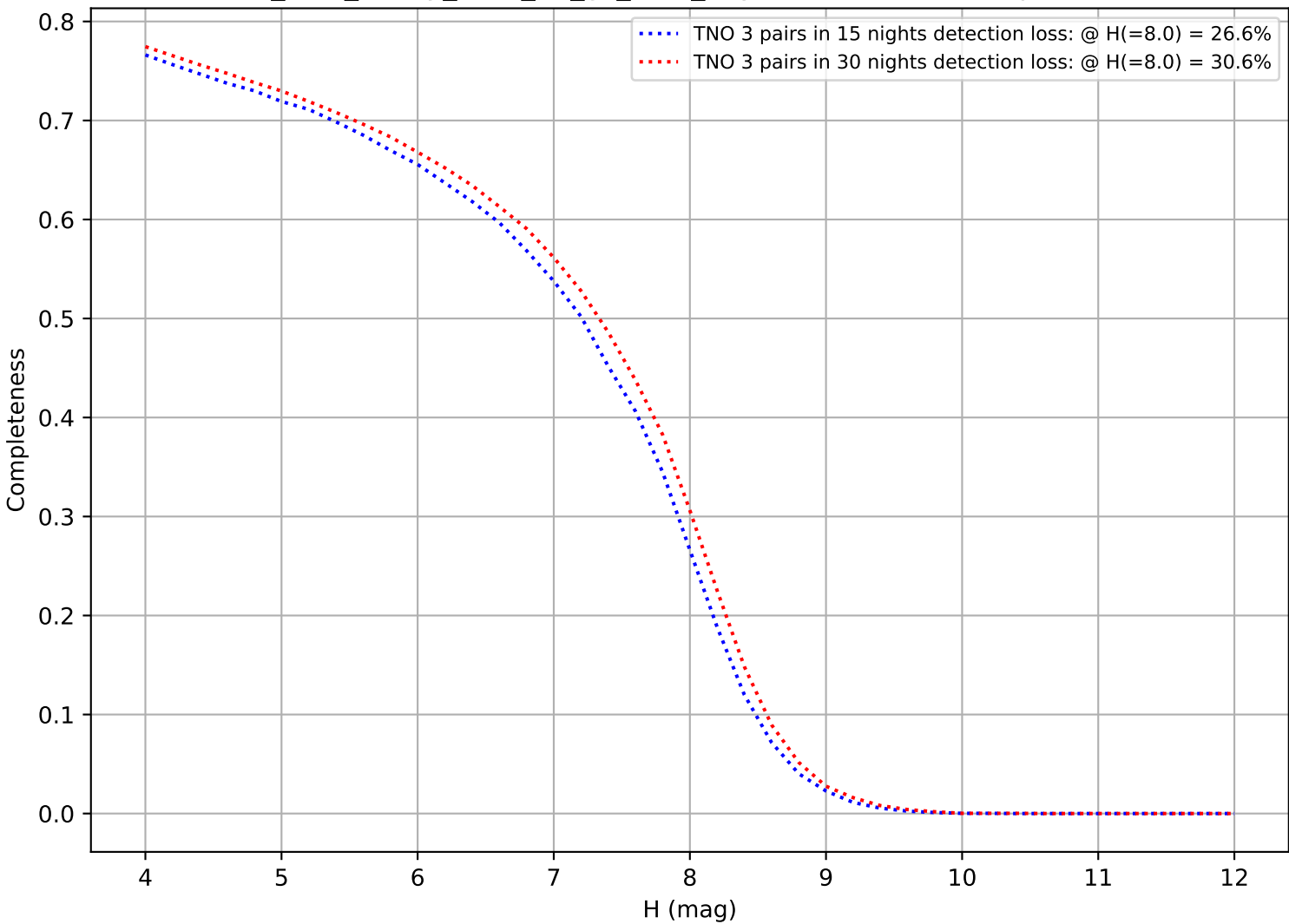
too_elab_heavy_r128_d2_gz_v3.4_10yrs: DifferentialCompleteness
