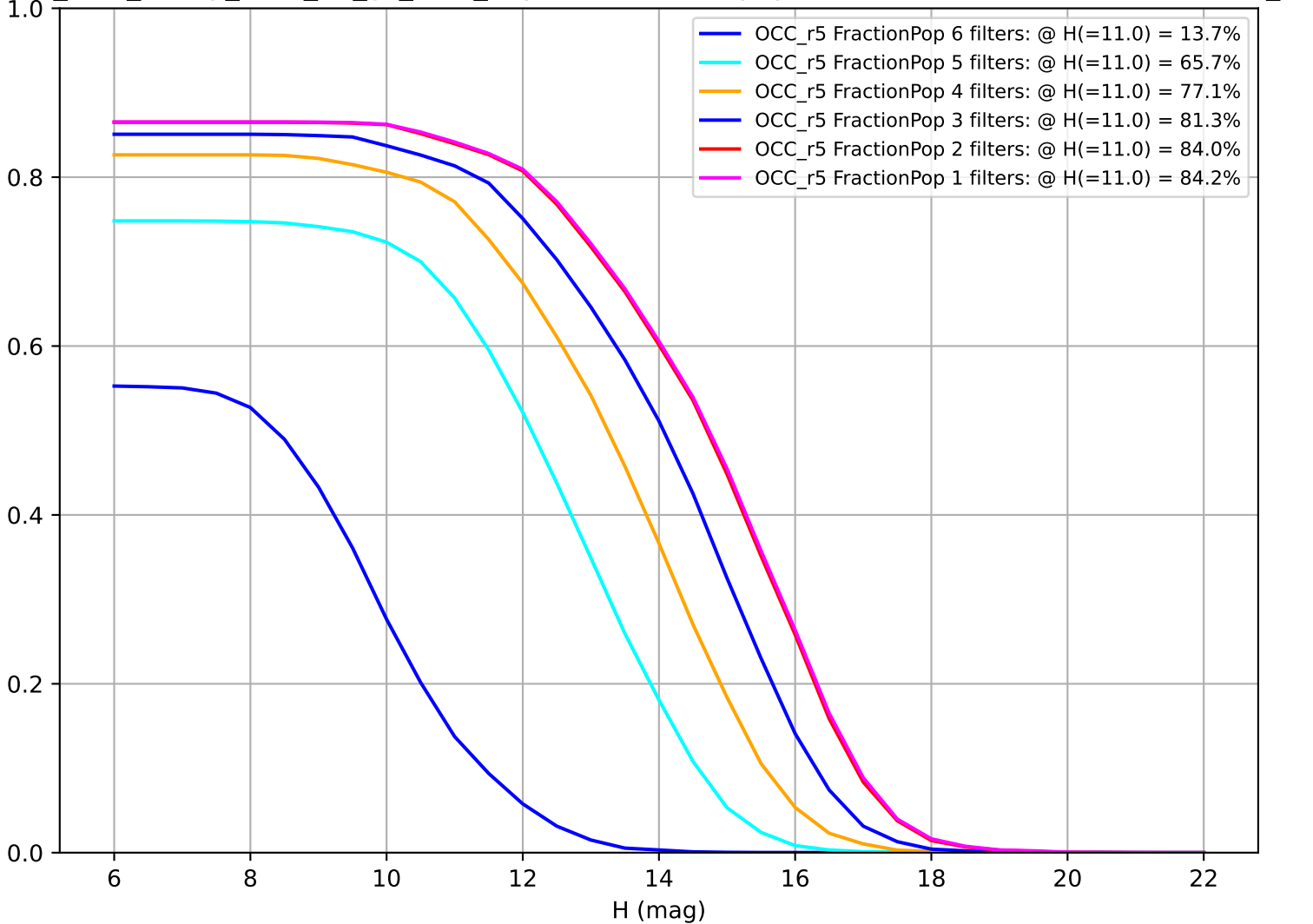
too_elab_heavy_r128_d2_gz_v3.4_10yrs: Fraction of population with colors in X filters OCC_r5
