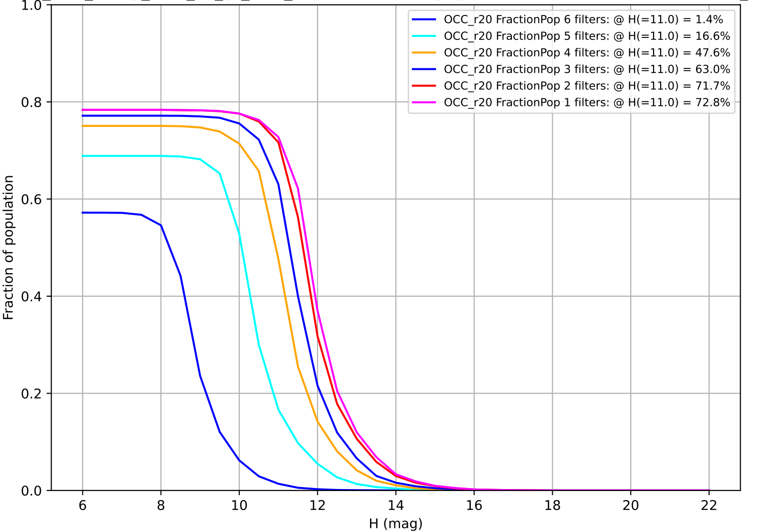
too_elab_heavy_r128_d2_gz_v3.4_10yrs: Fraction of population with colors in X filters OCC_r20
