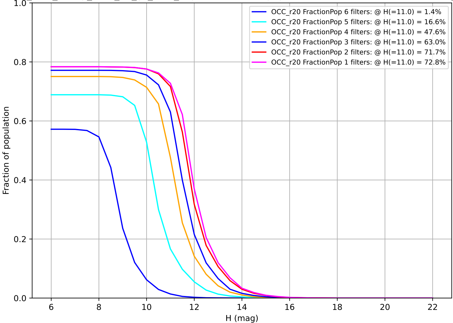
too_elab_heavy_r128_d2_gz_v3.4_10yrs: Fraction of population with colors in X filters OCC_r20
