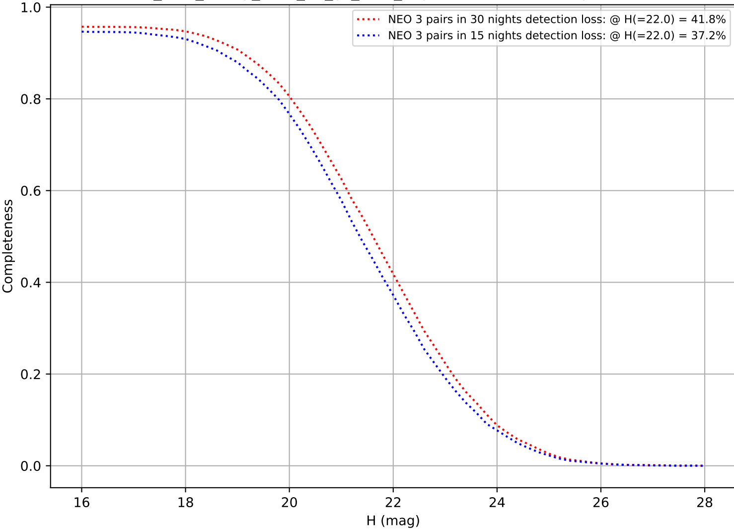
too_elab_heavy_r128_d2_gz_v3.4_10yrs: DifferentialCompleteness
