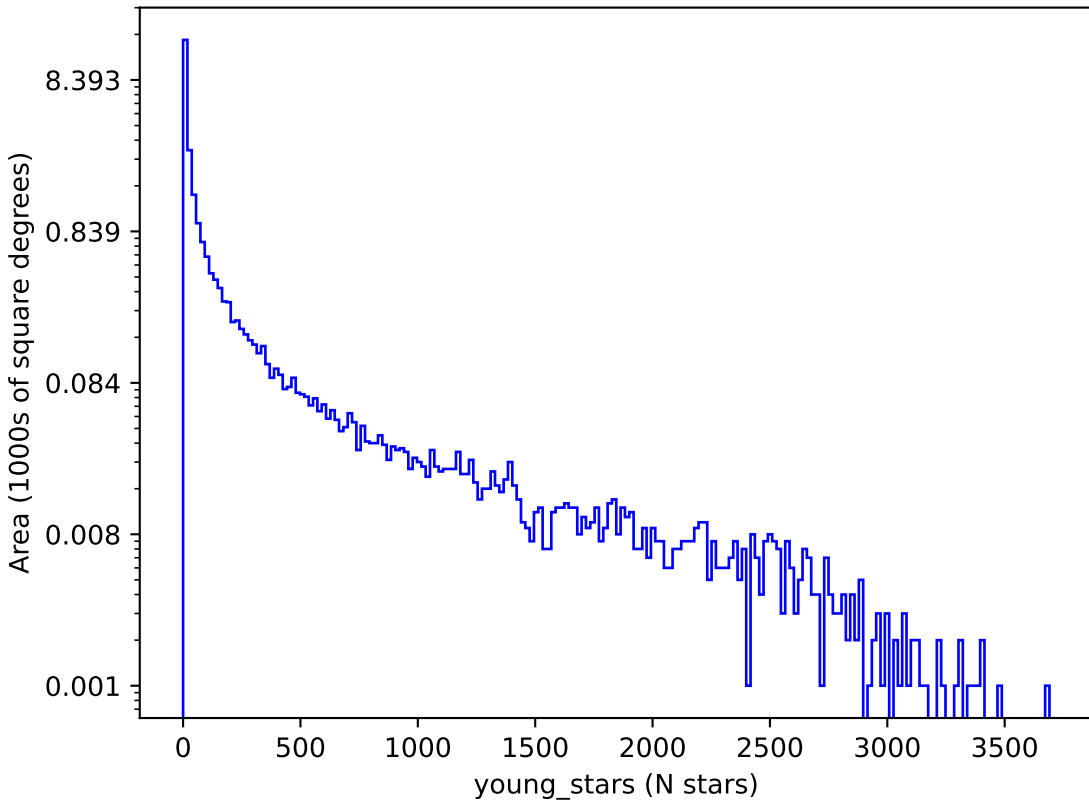
too_elab_heavy_r128_d2_gz_v3.4_10yrs : young_stars
