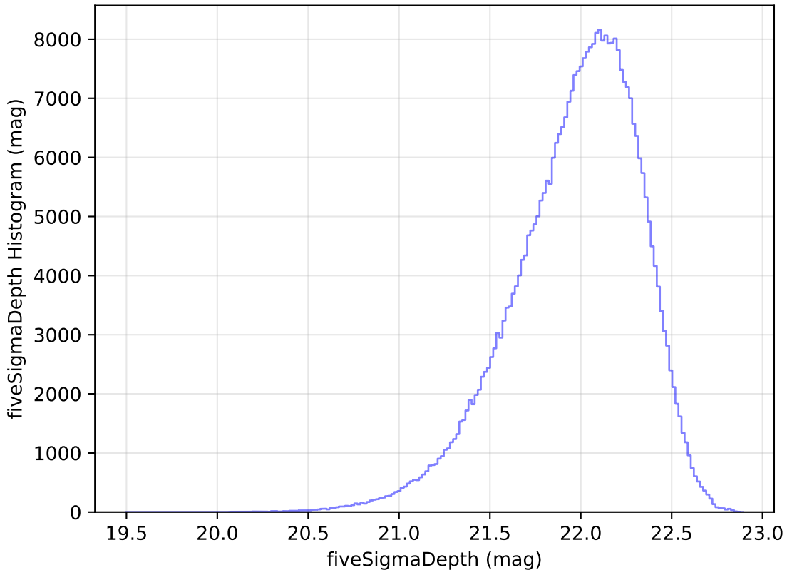
too_elab_heavy_r128_d2_gz_v3.4_10yrs y: fiveSigmaDepth Histogram
