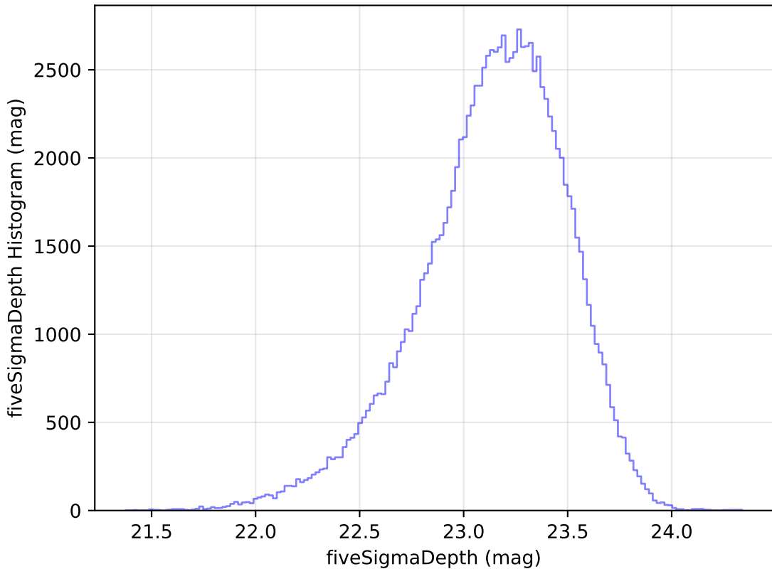
too_elab_heavy_r128_d2_gz_v3.4_10yrs u: fiveSigmaDepth Histogram
