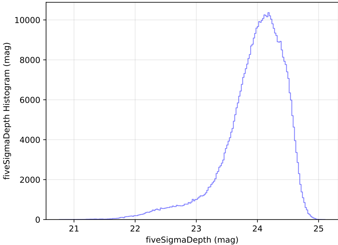
too_elab_heavy_r128_d2_gz_v3.4_10yrs r: fiveSigmaDepth Histogram
