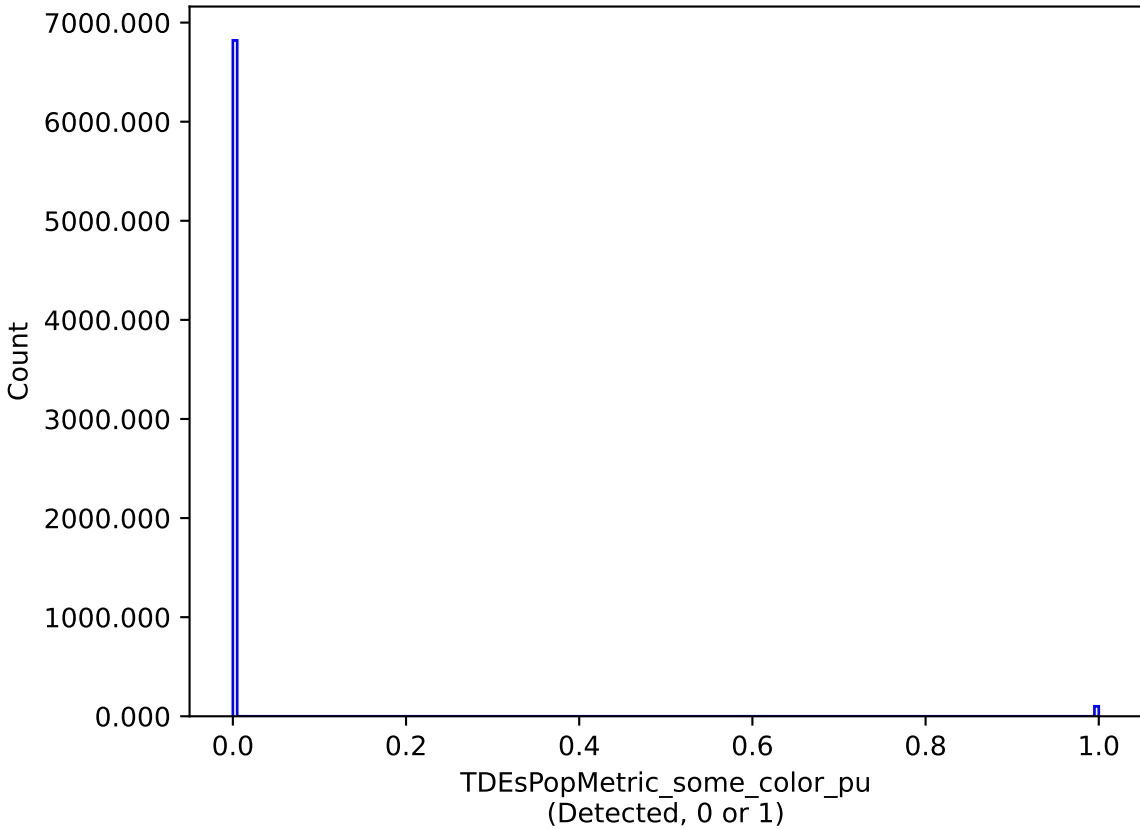
too_elab_heavy_r128_d2_gz_v3.4_10yrs : TDEsPopMetric_some_color_pu
