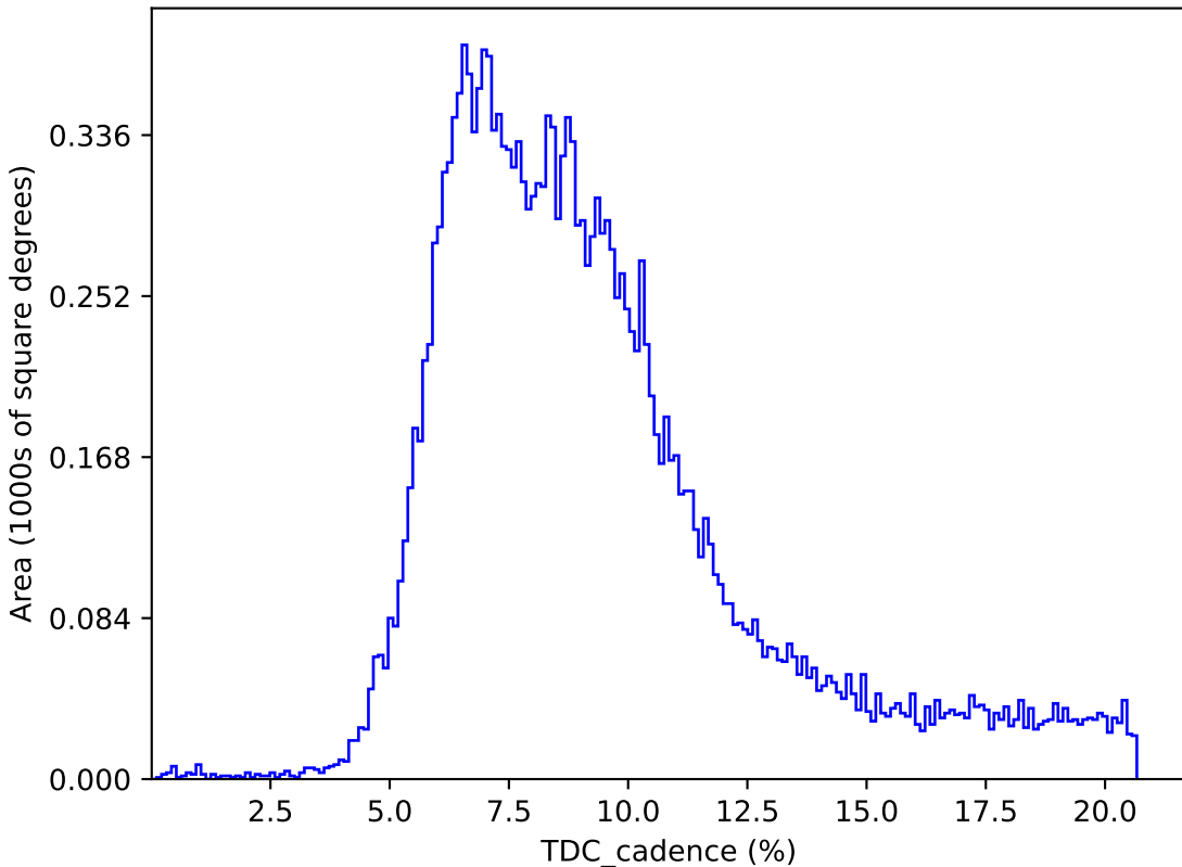
too_elab_heavy_r128_d2_gz_v3.4_10yrs : TDC_cadence
