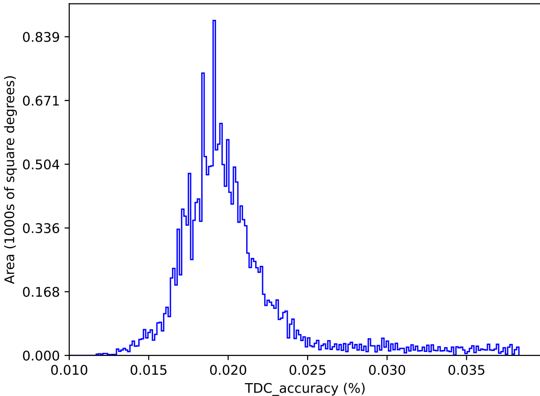
too_elab_heavy_r128_d2_gz_v3.4_10yrs : TDC_accuracy
