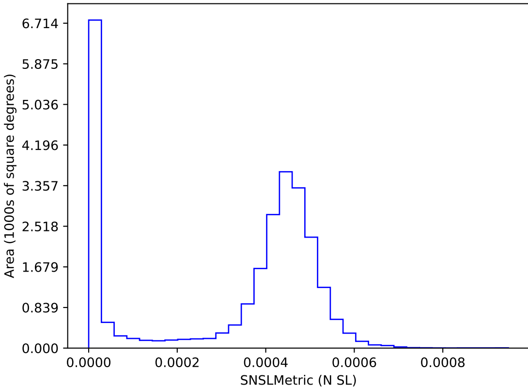
too_elab_heavy_r128_d2_gz_v3.4_10yrs : SNSLMetric
