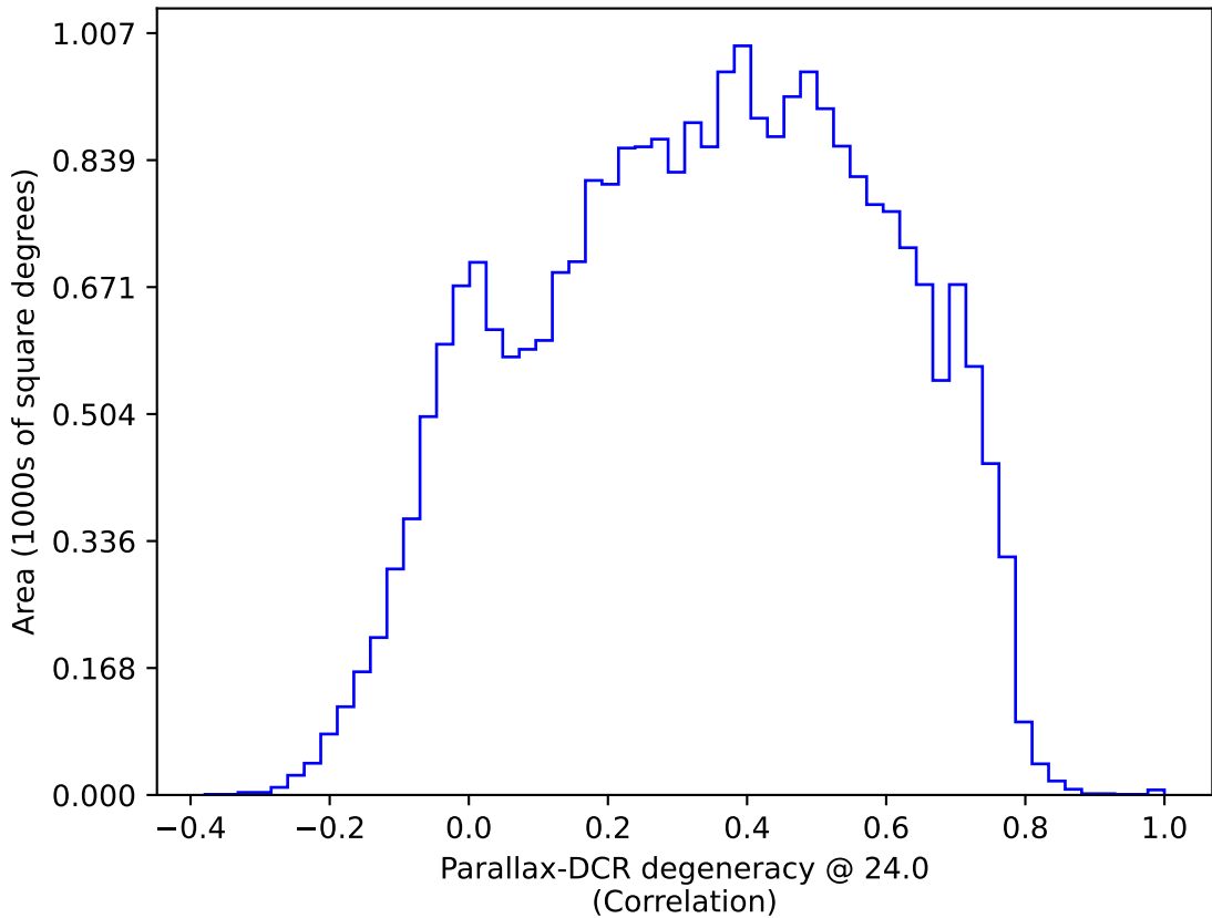
too_elab_heavy_r128_d2_gz_v3.4_10yrs : Parallax-DCR degeneracy @ 24.0
