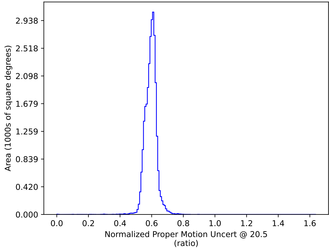
too_elab_heavy_r128_d2_gz_v3.4_10yrs : Normalized Proper Motion Uncert @ 20.5
