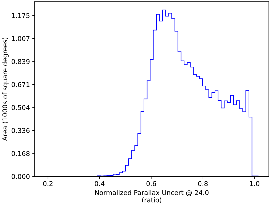
too_elab_heavy_r128_d2_gz_v3.4_10yrs : Normalized Parallax Uncert @ 24.0
