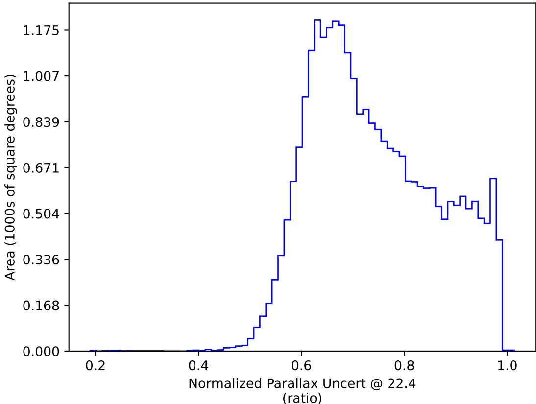
too_elab_heavy_r128_d2_gz_v3.4_10yrs : Normalized Parallax Uncert @ 22.4
