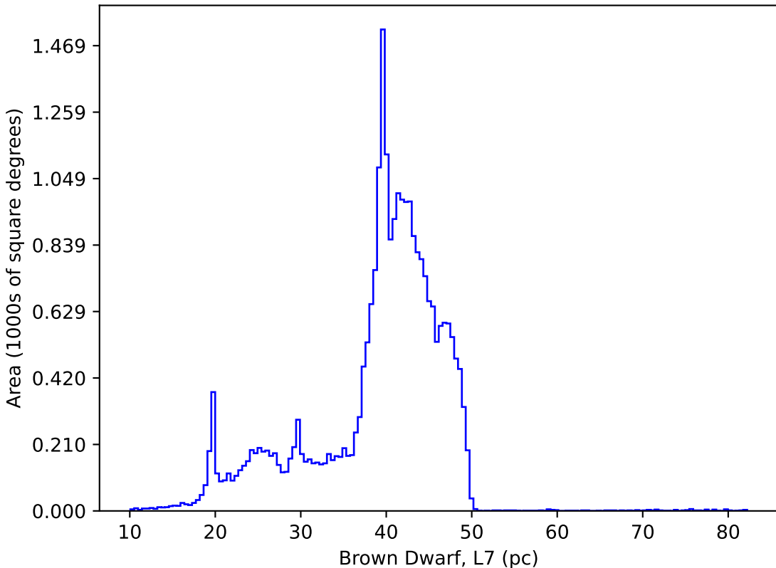
too_elab_heavy_r128_d2_gz_v3.4_10yrs : Brown Dwarf, L7
