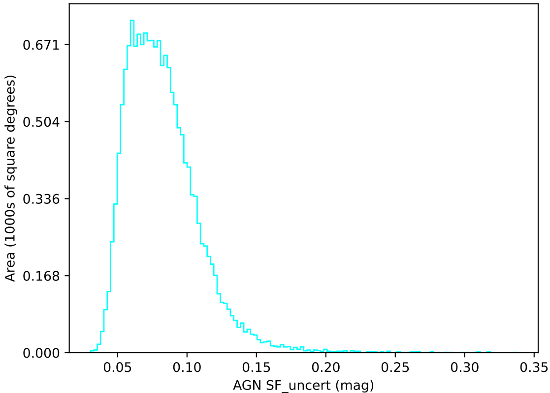
too_elab_heavy_r128_d2_gz_v3.4_10yrs u band: AGN SF_uncert
