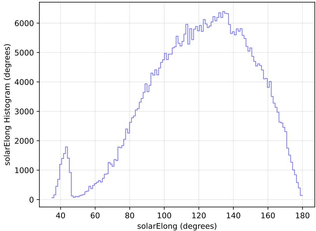
too_elab_heavy_r128_d2_gz_v3.4_10yrs WFD z band: solarElong Histogram
