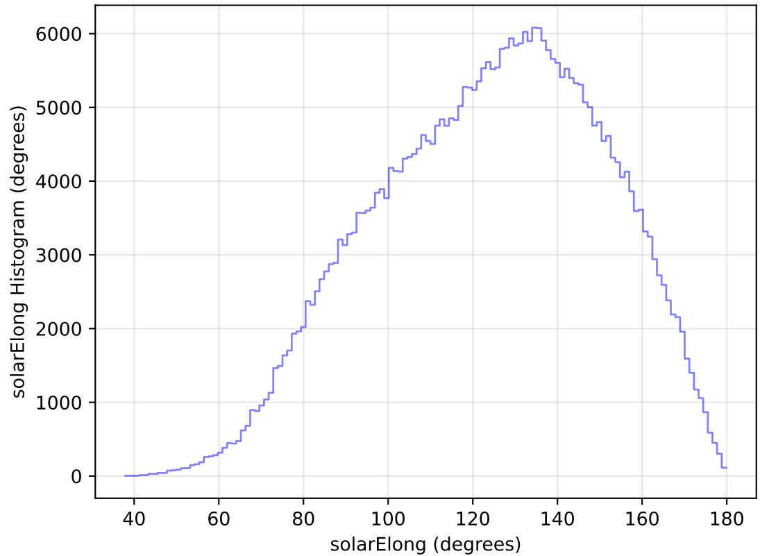
too_elab_heavy_r128_d2_gz_v3.4_10yrs WFD y band: solarElong Histogram
