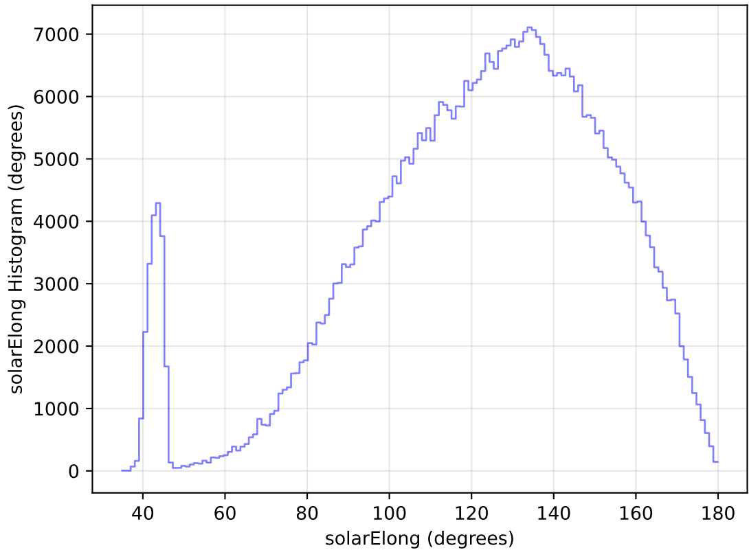
too_elab_heavy_r128_d2_gz_v3.4_10yrs WFD r band: solarElong Histogram
